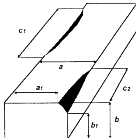
Figure 15. Wane
