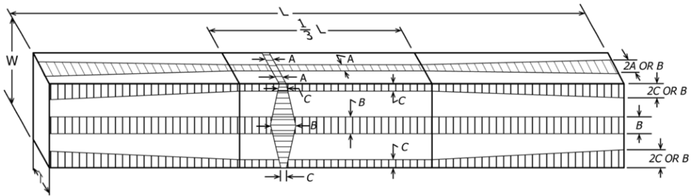
FIG. 3 Maximum Size of Knots Permitted in Various Parts of Joists and Planks, and Beams and Stringers A, maximum size on narrow face in middle third of length with a uniform increase to 2A but not to exceed B , at the ends. B, maximum size at center of wide face. C, maximum size at edge of wide face in middle third of length with a uniform increase to 2C but not to exceed B at the ends and a uniform increase to B at the center of the wide face. In beams and stringers, A and C are equal. L, length. W, width of wide face. T, width of narrow face.
