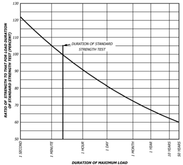
FIG. 6 Relation of Strength to Duration of Load
