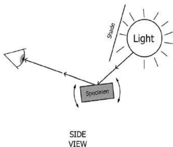
FIG. 2 Positioning of Test Specimen in Relation to Light Source and Eye
