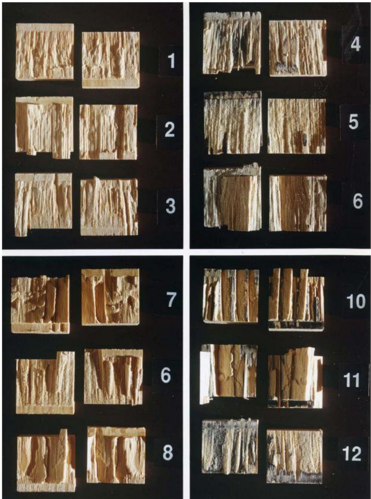
FIG. X1.3 Visually Estimating the Percentage of Wood Failure in Standard Adhesively Bonded Specimens
