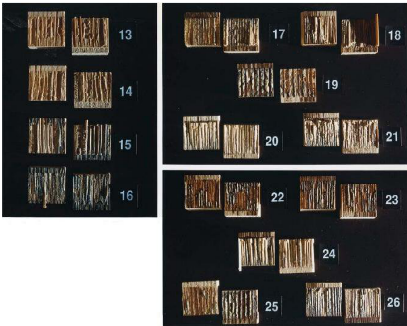
FIG. X1.4 Visually Estimating the Percentage of Wood Failure in Standard Adhesively Bonded Specimens
